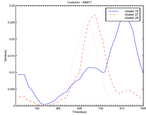
Figure 8. A plot of similarity between three clusters; 15, 27 & 29 for customer 306671 showing customer drift across time. A clear correlation can also be seen between clusters 27 & 29.
