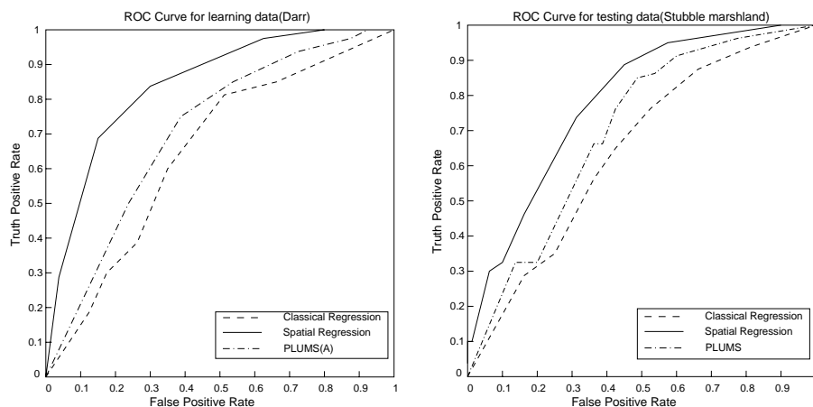
(a) ROC curves for Learning Data
