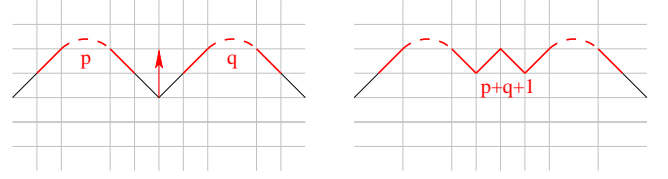
Figure 7: An irreversible flip which replaces two maximal Dyck factors with respectively p and q letters 1 by a single maximal Dyck factor with p+q+1 letters 1.
