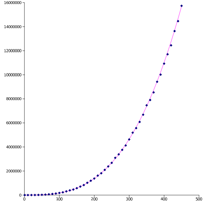
Figure 9: The blue points represent the average over 10 simulations of the worst convergence time (on the x -axis, the length n of configurations). The pink curve has equation n \rightarrow 0.17n^3 .
