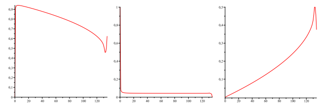
Figure 6: Left, the probability that the singular Boltzmann sampler \Gamma\mathcal{P}^{(k,135)} of objects in \mathcal{P}^{(k,135)} stops immediately. Middle, the probability that the sampler \Gamma\mathcal{P}^{(k,135)} calls \Gamma\mathcal{P}^{(k-1,135)} . Right, the probability that the sampler \Gamma\mathcal{P}^{(k,135)} independently calls 2 generators \Gamma\mathcal{P}^{(k,135)} .
