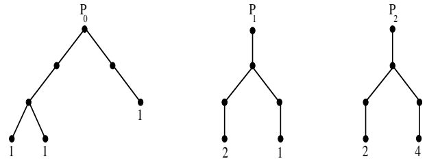
Figure 2: The trees P_0 and P_1 are elements of \mathcal{P}^{(0, 2)} \cong \mathcal{S}^{(2)} and correspond to T_0 and T_1 in Fig. 1. The tree P_2 is an element of \mathcal{P}^{(i, 2)} for i \geq 2 : Both leaves have the same unary height as the tree itself, namely 2, and the label of the right (resp. left) leaf exceeds its unary height by 2 (resp. 1). Thus P_2 \notin \mathcal{P}^{(i, 2)} for i < 2 .
