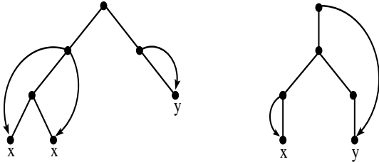
Figure 1: Two examples of lambda-terms: Each unary node corresponds to an abstraction \lambda x binding all leaves below it which are labelled by x . Binary nodes correspond to applications merging their two subtrees t_1 and t_2 to the more complex structure t_1 * t_2 .
