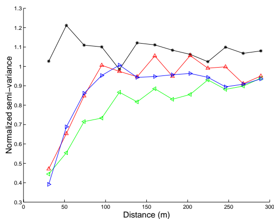
Figure 4. Semi-variogram comparison of simulated uncorrelated noise (-*-) and ordinary linear regression residuals on data generated with non-linear homogeneous DGP for three time instants: t=3 ( \rightarrow ), t=4 ( \Delta ) and t=5 ( \leftarrow ).
