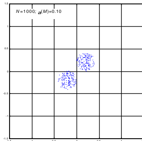
Fig.2b. A data-set with 1000 data-points.
