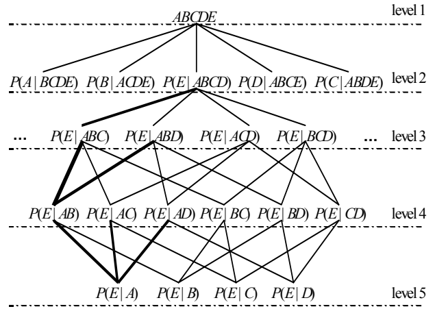
Figure 3.1. A Possible Semi-lattice for the Frequent Itemset ABCDE.
