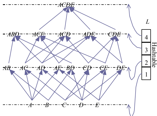
Figure 3.6. A Semi-Lattice for All Frequent Itemsets
