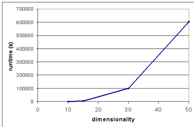
Figure 7: Scalability of SUBCLU against the dimensionality of the dataset.
