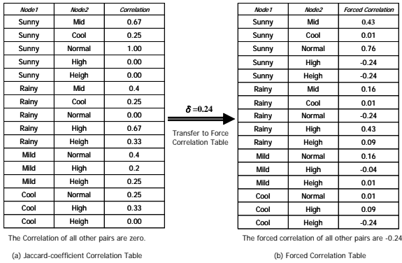
Figure 4: The Force Correlation table.
