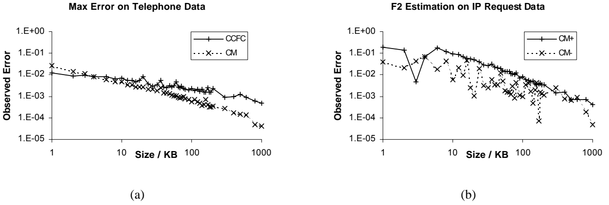
Figure 5: Results of experiments on network data
