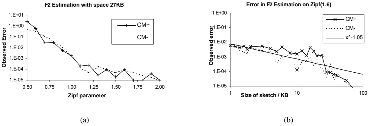
Figure 3: Testing space L_2 estimation on synthetic data
