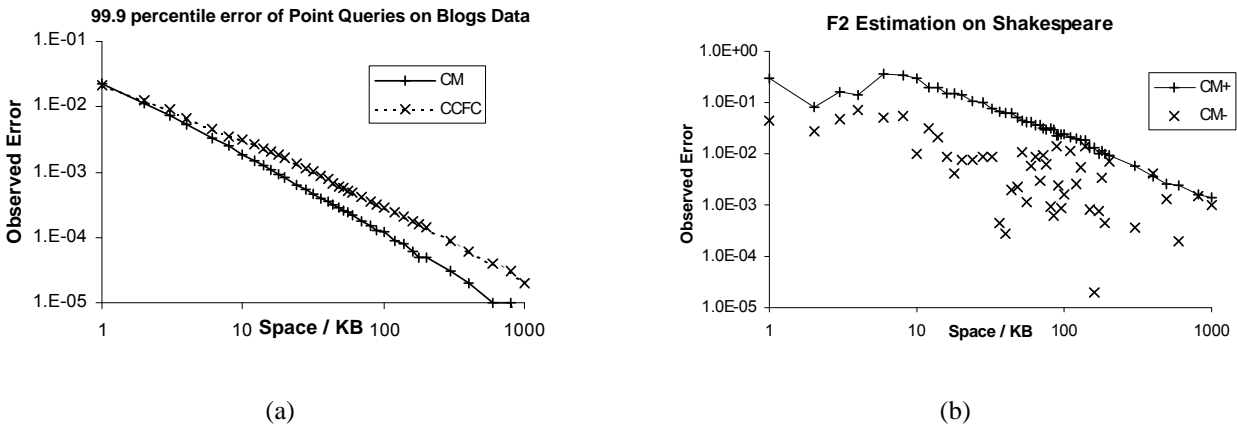
Figure 4: Results of experiments on text data
