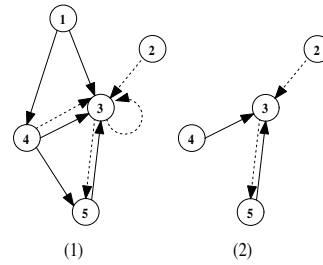
Figure 3: Frequent Graphs
