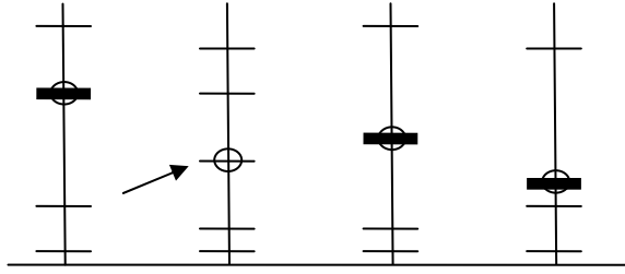
Figure 1: Graphical representation of our MN algorithm. Vertical lines are dimensions, horizontal lines are values (thick horizontal lines are the same value occurring twice), and circles are current cluster center locations. Sliding the second circle upward incurs less error than sliding any other circle would since more values are above it.
