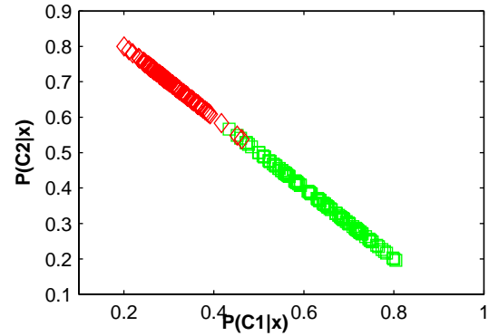
Figure 6: Two dimensional probability vectors P = (P(C_1|\mathbf{x}), P(C_2|\mathbf{x}))^t , (1/h) = 12 . LAC error rate is 5.3%.
