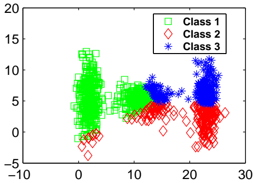
Figure 8: LAC: Clustering results for Three-Gaussian data, (1/h) = 1 . The error rate is 34.6%
