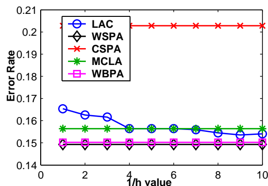
Figure 16: Results on SatImage dataset
