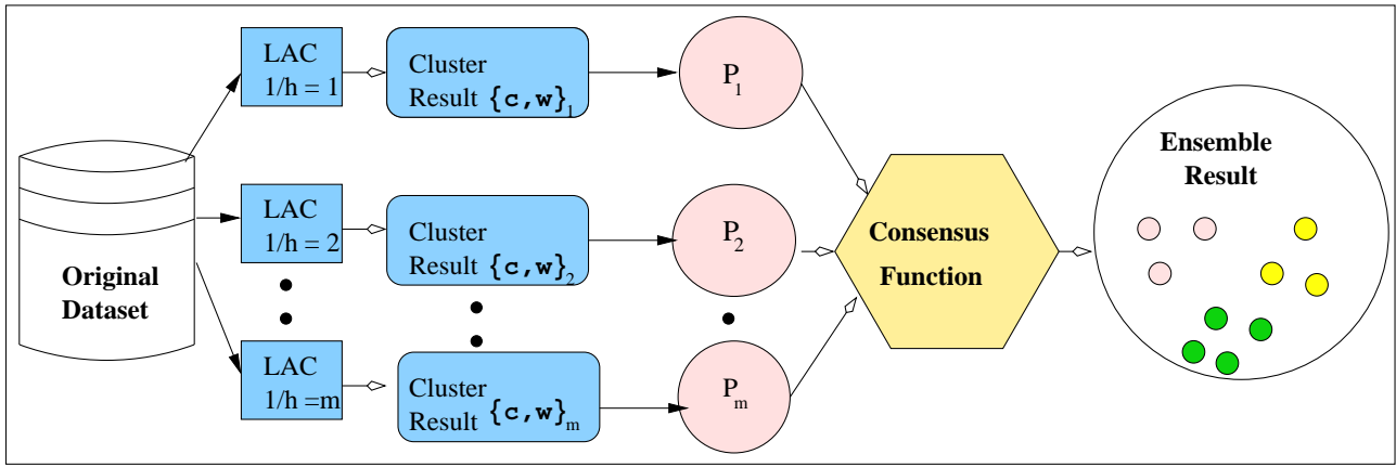
Figure 1: The clustering ensemble process
