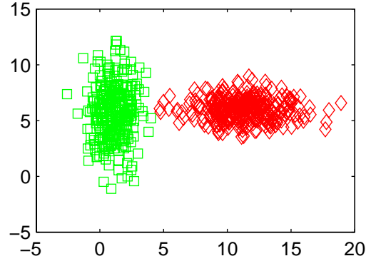
Figure 2: Two-Gaussian data
