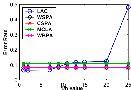
Figure 15: Results on Letter (A,B) dataset
