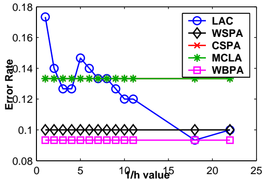
Figure 11: Results on Iris data
