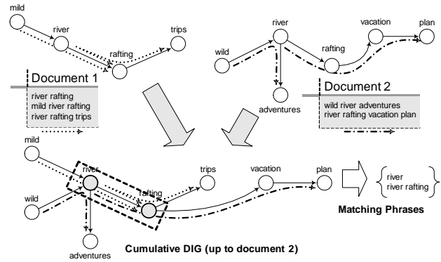
Figure 3: Phrase Matching Using Document Index Graph
