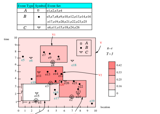
Figure 2: Concept Illustration: Density of B events in different regions
