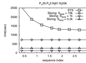
(a) Performance w.r.t Sequence Index
