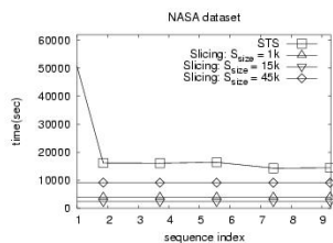
(e) Performance w.r.t. Sequence Index Thresholds
