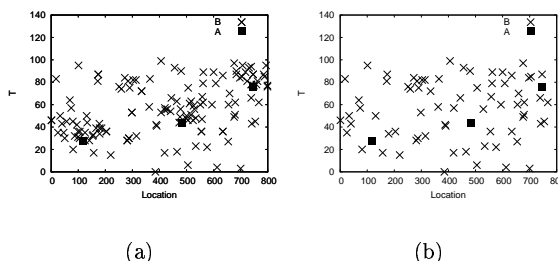
Figure 1: (a) B follows A (b) B is independent of A
