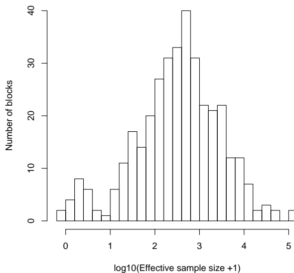
Figure 5: Estimated effective sample sizes ( \gamma ) for blocks.
