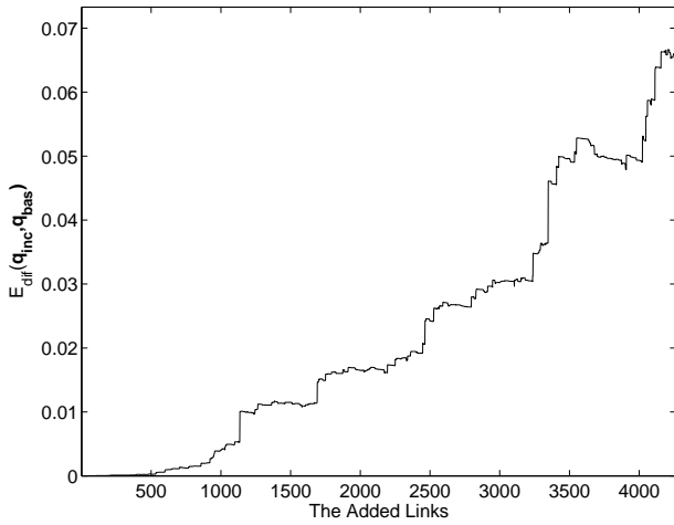
Figure 5: The error E_{diff}(\mathbf{q}_{inc}, \mathbf{q}_{bas}) of the eigenvectors with the second smallest eigenvalue.
