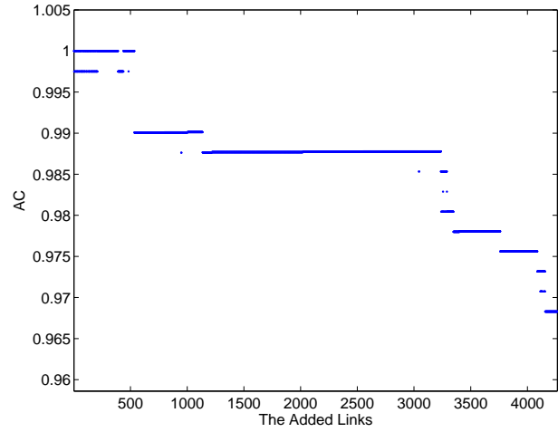
Figure 7: The accuracy corresponding to each added link.
