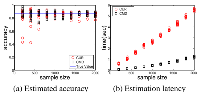
Figure 14: Accuracy Estimation: (a) The estimated accuracy are very close to the true accuracy; (b) Accuracy estimation performs much faster for CMD than CUR
