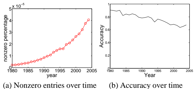
(a) Nonzero entries over time (b) Accuracy over time Figure 17: DBLP over time: The approximation accuracy drops slowly as the graphs grow denser.
