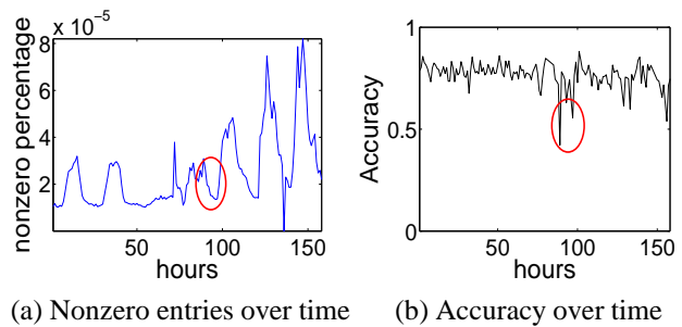
(a) Nonzero entries over time (b) Accuracy over time Figure 16: Network flow over time: we can detect anomalies by monitoring the approximation accuracy (b), while traditional method based on traffic volume cannot do (a).
