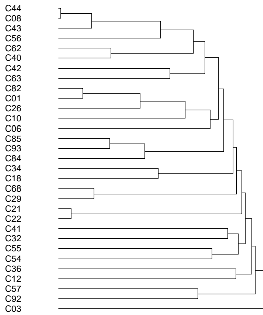
Figure 1: Dendrograms for hierarchical clustering using the N_{\chi^2} measure.
