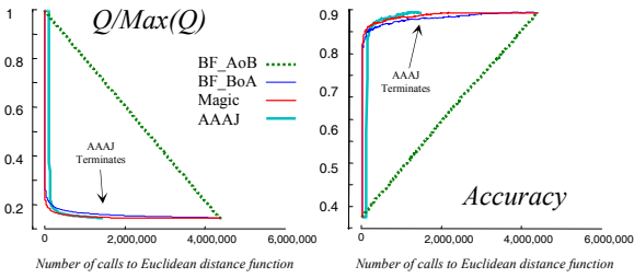
Figure 4: (Left) The normalized value of Q as a function of the number of calls to the Euclidean distance. (Right) The accuracy of classification, averaged over the 30 unknown letters, as a function of the number of calls to the Euclidean distance.
