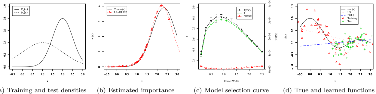
Figure 1: Regression under covariate shift.
