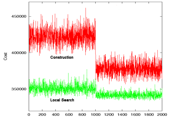
Figure 9: One execution of DM-GRASP.
