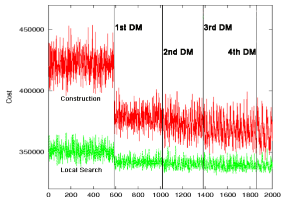
Figure 10: One execution of MDM-GRASP.
