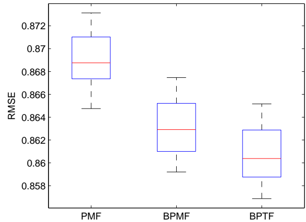
Figure 7: Box plot of the accuracies from PMF, BPFM, and BPTF on MovieLens data.
