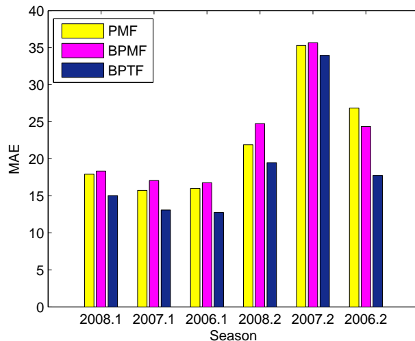
Figure 3: Performance comparison of PMF, BPFM, and BPTF on 6 seasons of ECCO data. BPTF outperforms others by a large margin. See text for details.
