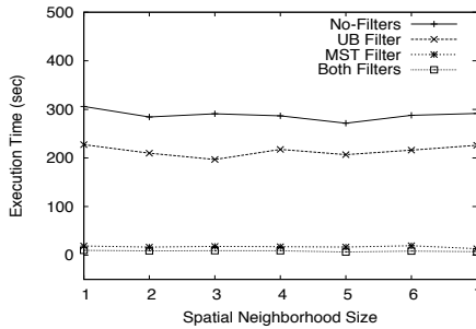
Figure 15: Effect of Spatial Neighborhood Size(Execution times range from 7.022 to 19.418 seconds)
