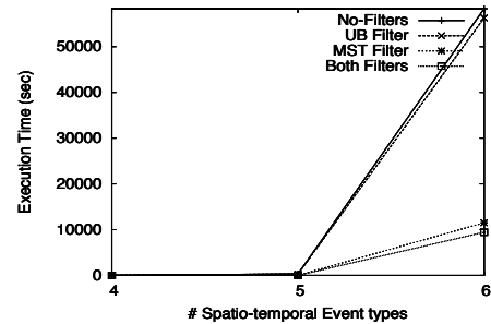
Figure 13: Effect of # event types(Execution times range from 6.3695 to 11512 seconds)
