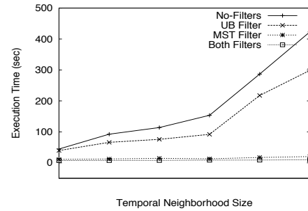
Figure 16: Effect of Temporal Neighborhood Size (Execution times range from 7.368 to 20.188 seconds)
