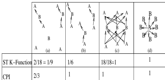
Figure 6: The CPI as an upper bound to the space-time K-Function[21]
