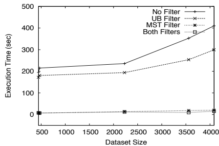
Figure 12: Effect of Dataset Size (Execution times range from 7.9170 to 20.2039 seconds)
