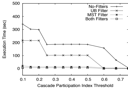
Figure 14: Effect of CPI Threshold(Execution times range from 4.0548 to 22.3895 seconds)
