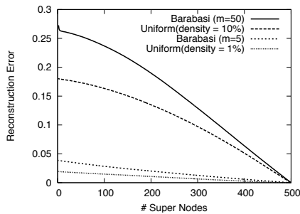
Figure 14: k -Gs, Barabasi-Albert(500)
