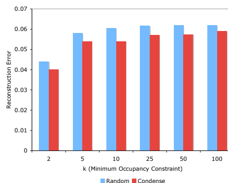
Figure 16: k -CGs, Italy(500)
