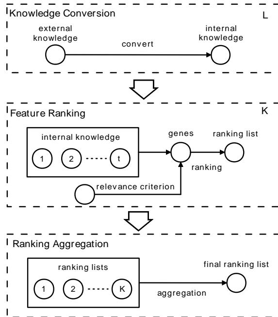
Figure 1: An approach for integrating different types of domain knowledge to assist gene selection.
