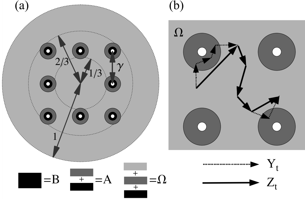
Figure 2: An illustration the sets \Omega , A and B (a), and a possible sequence of jumps in the processes \{Y_t\} and \{Z_t\} (b)
