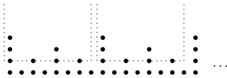
Figure 1: Proof of Lemma 4.1: the point set P and two level-1 rectangles (with b = 2 and k = 4 ).
