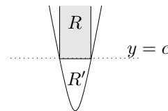
Figure 2: Proof of Theorem 4.1: the rectangle R = [a, b] \times [c, \infty) and the parabolic range R' = \{(x, y) : y - c \geq m(x - a)(x - b)\} . As m \rightarrow \infty , R' approaches the slab [a, b] \times \mathbb{R} .
