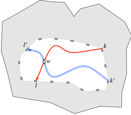
Figure 5: Nodes k < k' < l < l' in clockwise order on the boundary nodes. Paths from k to l and from k' to l' must cross at some node w . This is true both in the internal and the external subgraphs of G
