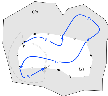
Figure 2: The solid blue path is an r -to- v shortest path in G . It can be decomposed into four subpaths. The subpaths P_1 and P_3 ( P_2 and P_4 ) are shortest paths in G_1 ( G_0 ) between boundary nodes. The r -to- v shortest paths in G_0 and G_1 are shown in gray in the background.
