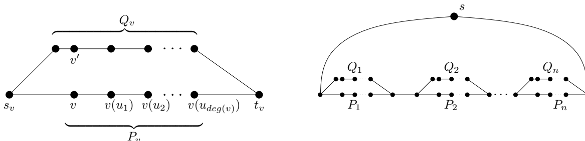
Figure 4: Reduction in Theorem 3.
