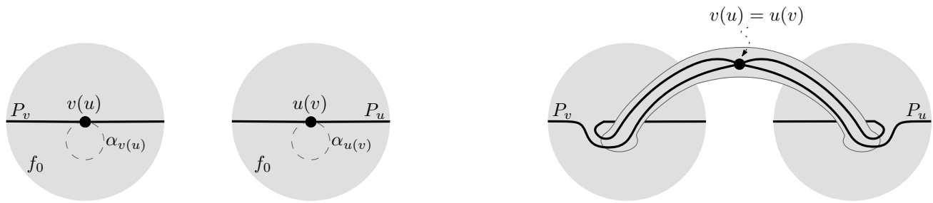
Figure 5: Illustration for the local transformation in the proof of Theorem 4. Left: part of the original graph G_H and two curves \alpha_{v(u)} and \alpha_{u(v)} . Right: part of the resulting surface \Sigma' after adding the handle corresponding to the edge uv of H .
