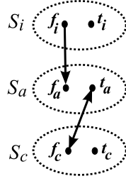
Figure 1: The copy gadget —in any Nash equilibrium \Pr[s(c) = f_c] = \Pr[s(i) = f_i] .
