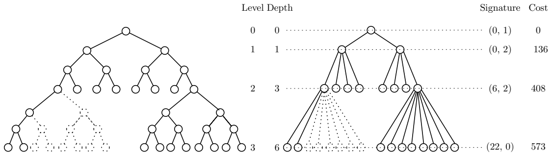
Figure 3: A Reserved-Length tree (left) with \Lambda = \{1, 3, 6\} , n = 16 leaves and the corresponding GMR tree (right). Note that even though they are allowed, there are no leaves on level 1. All internal nodes on level 3 should have 8 descendents on level 6 so 6 leaves were added to make the tree full. Signatures and costs for the GMR tree at level i are for the truncated tree containing the first i levels. Costs are for P = \{1, 2, \dots, 16\} .
