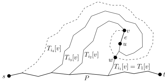
Figure 5: Path T_{i_4}[v] must leave T_1[v] from the left at a vertex w after entering this path from the right. But this contradicts the right-shortness of T_{i_4}[v] .
