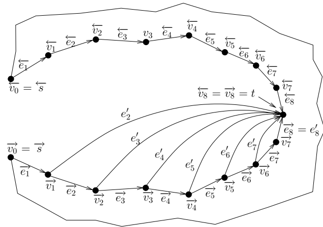
Figure 10: Graph G' , obtained from G in phase 2 by adding edges e'_i for i = 2, \dots, m - 1 , here shown for an instance with m = 8 .
