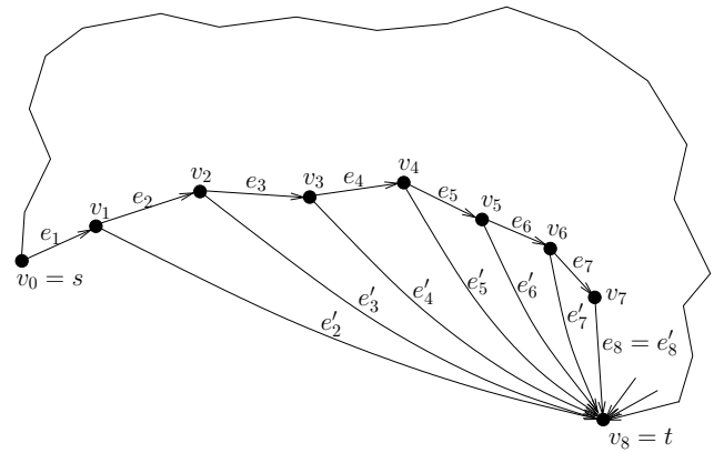
Figure 6: Graph G' is obtained from G by adding edges e'_i for i = 2, \dots, m-1 , here shown for an instance with m = 8 .
