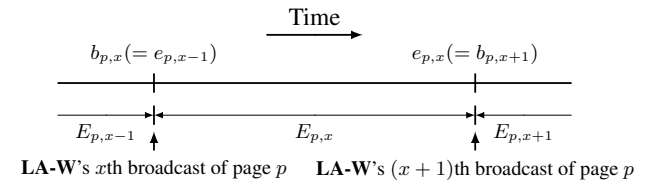
Figure 2: Events for page p .
