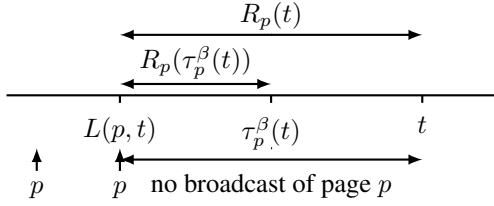
Figure 1: R_p(t) denotes the alive requests of page p at time t , i.e. the requests of page p which arrived during [L(p, t), t] . Likewise, R_p(\tau_p^\beta(t)) denotes the requests which arrived during [L(p, t), \tau_p^\beta(t)] .
